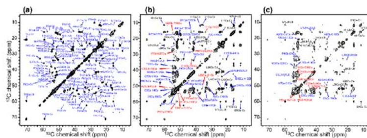
Figure 8. 2D ^{13}\text{C} - ^{13}\text{C} DARR spectra of HNP-1 with mixing times (a) 40 ms, (b) 100 ms, and (c) 200 ms. In (a), all peaks are assigned. In (b) and (c), only inter-residue and intra-residue multiple-bond correlations not observed in (a) are assigned. Red: non-sequential inter-residue correlations; blue: sequential correlations; black: intra-residue multiple-bond correlations.
