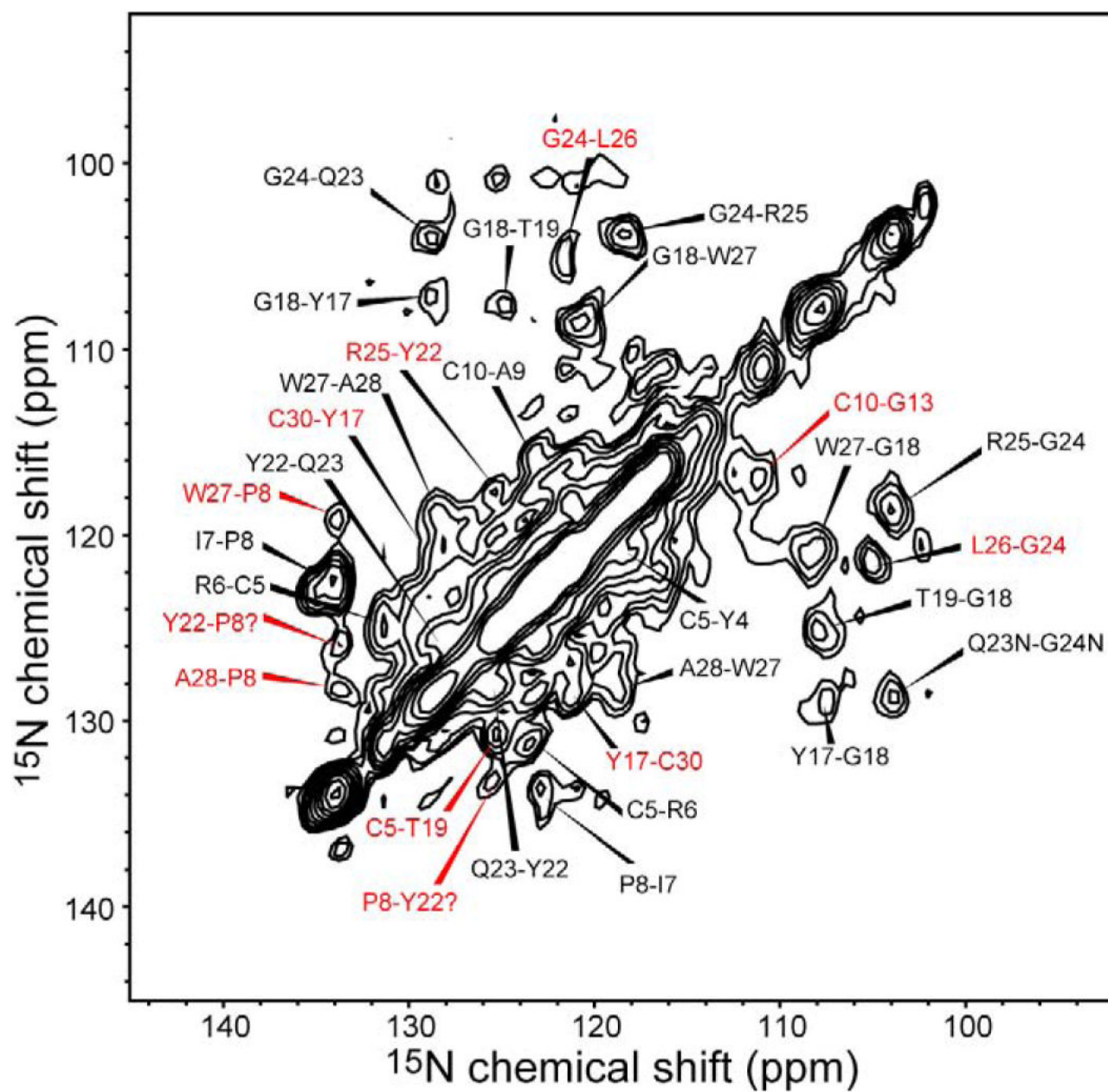
Figure 9. ^{15}\text{N} - ^{15}\text{N} 2D PDSD spectrum with a mixing time of 3 s. Black and red assignments indicate sequential and non-sequential correlations, respectively.
