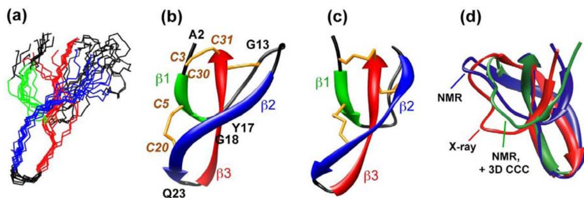
Figure 10. SSNMR structures of HNP-1 compared with the X-ray crystal structure of HNP-3. (a) Eleven minimum energy SSNMR structures of HNP-1. (b) Average structure of (a). (c) Crystal structure of HNP-3. The disulfide bonds are shown in orange. (d) Comparison of the \beta1 - \beta2 loop conformation between the crystal structure (red), the current solid-state NMR structure (blue), and the NMR structure with the additional distance restraints from the 3D CCC experiment (green).
